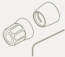
Pro Tail Cover kit (Prop C only) Pro Tail Cover, Ring Nut Tool, 2.5mm hex key & 13mm socket
